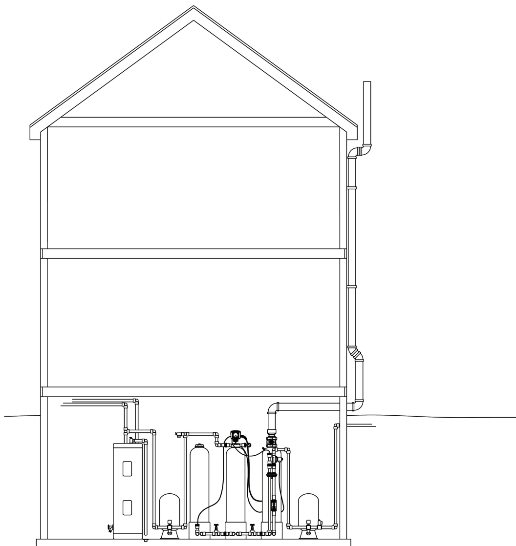
TYPICAL RADON VENTING DIAGRAM
